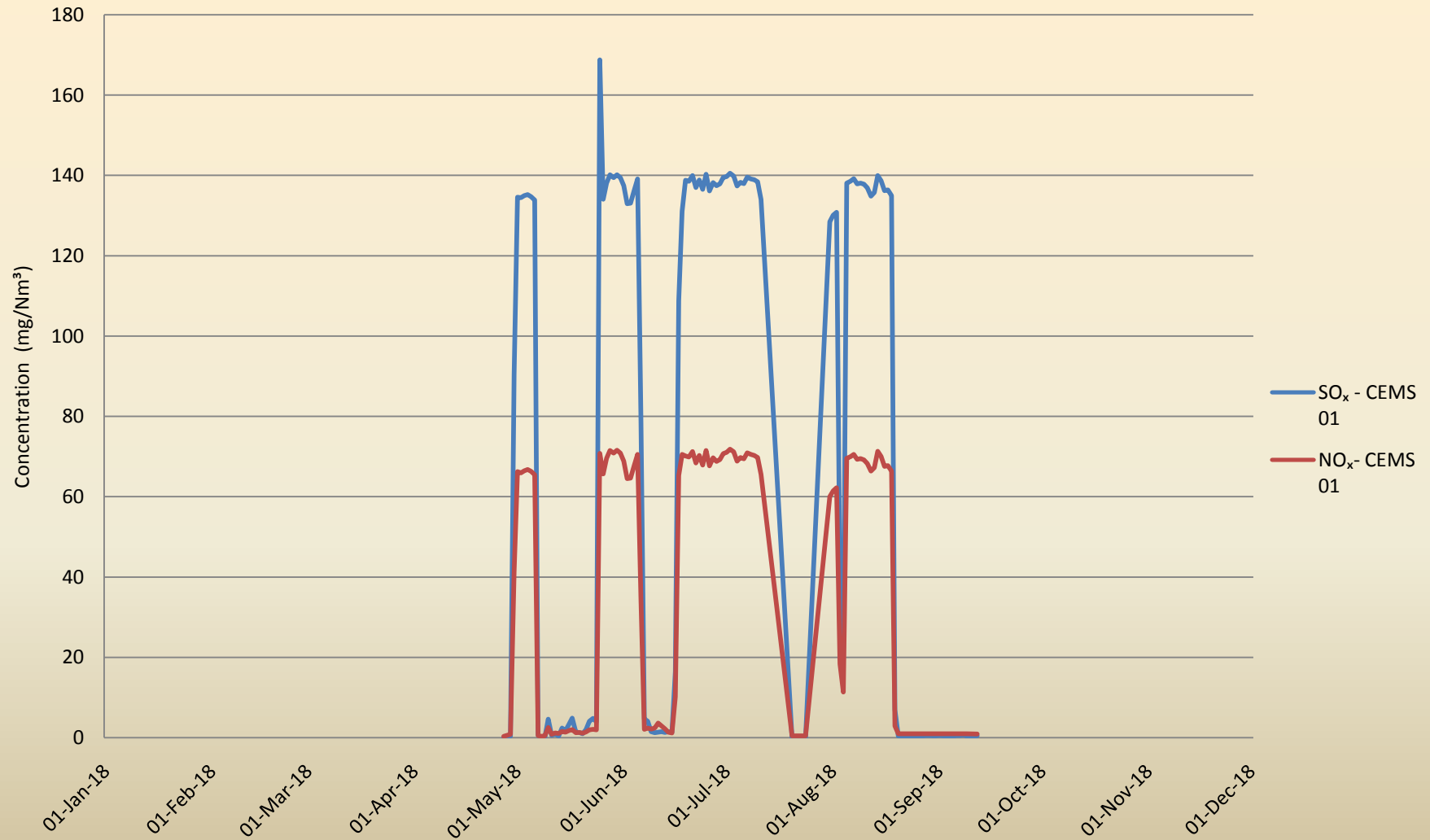
Annual Emission Trend of Gaseous in M/s. BLA Power (P) Ltd., Dist. Narsinghpur (M.P.)
